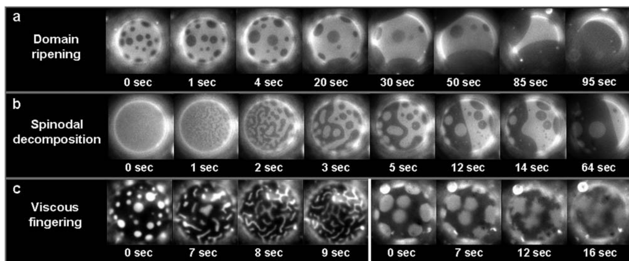
FIGURE 3 Giant vesicles observed near the miscibility transition. (a) Domain ripening through time in a vesicle of 1:1 DOPC/DPPC + 25% Chol. Although the proportion of dark phase increases in one hemisphere, it is roughly constant in time over the entire vesicle. (b) Time sequence suggesting spinodal decomposition in a vesicle of 1:1 DOPC/DPPC + 35% Chol. (c) Viscous fingering in a vesicle of 1:9 DOPC/DPPC + 25% Chol (left series) and 1:1 DOPC/DMPC + 25% Chol (right series) as temperature is raised through the miscibility transition. The uniform stripe-widths shown at the left are unique to this vesicle composition. All vesicles are roughly 30 \mu\text{m} in diameter.
